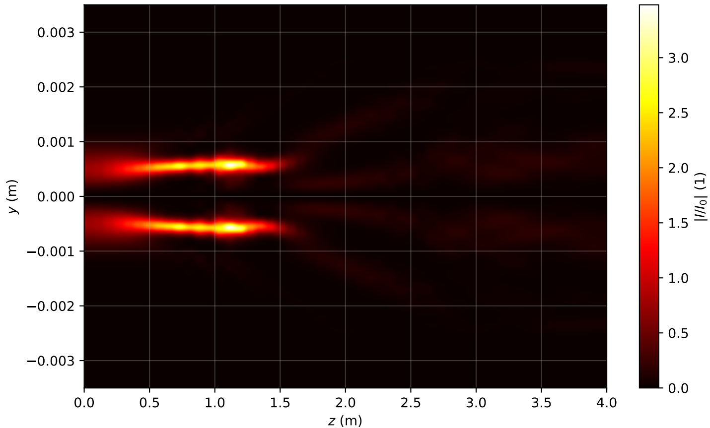
Intensity profile I(x=0, y, z)/I_0 , P_{in}=9.0P_{cr} , artificial time
